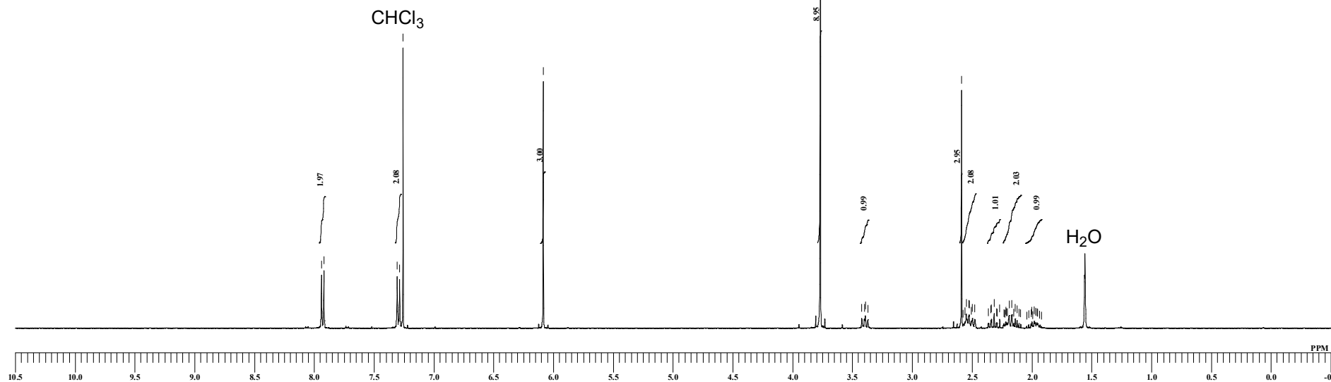
1,3,5-trimethoxybenzene (internal standard)
