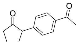
2-(4-acetylphenyl)cyclopentan-1-one ( 4 ) 1 H NMR (400 MHz, CDCl 3 )
